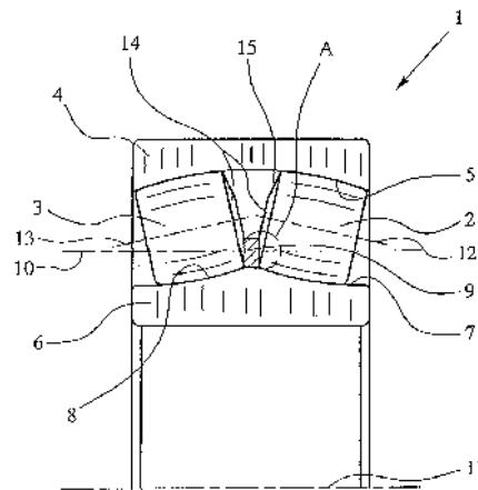
Figure 3: Exemplar State Of The Art Bearing System.
