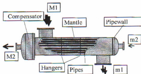
Figure 1: Heat Exchanger Arrangement
