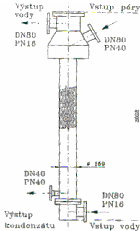
Figure 7: CZ 280 320 B6 Heat Exchanger
