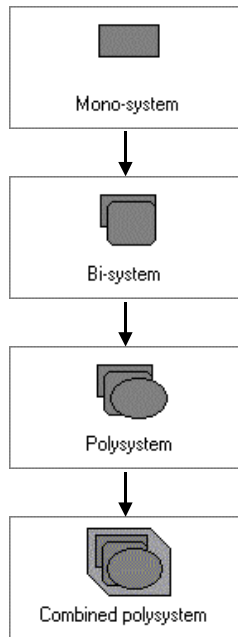
Figure 6: ‘Mono-Bi-Poly’ Trend
